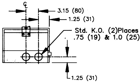
Aluminum Enclosure
